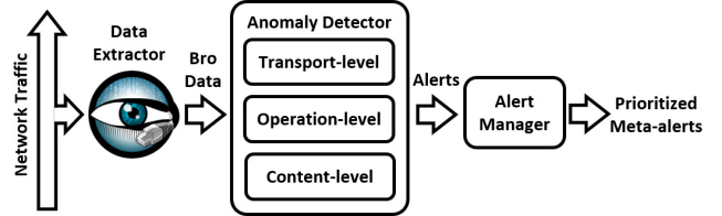
Fig. 2. EDMAND architecture
