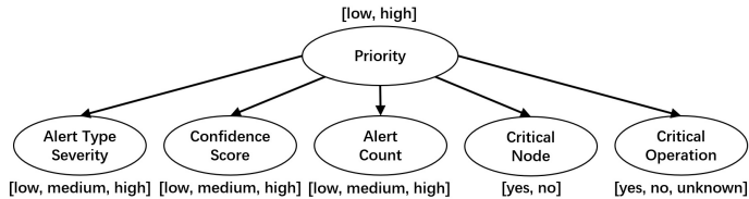
Fig. 7. Alert priority computation model
